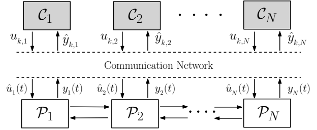
Fig. 1. Decentralized NCS.
