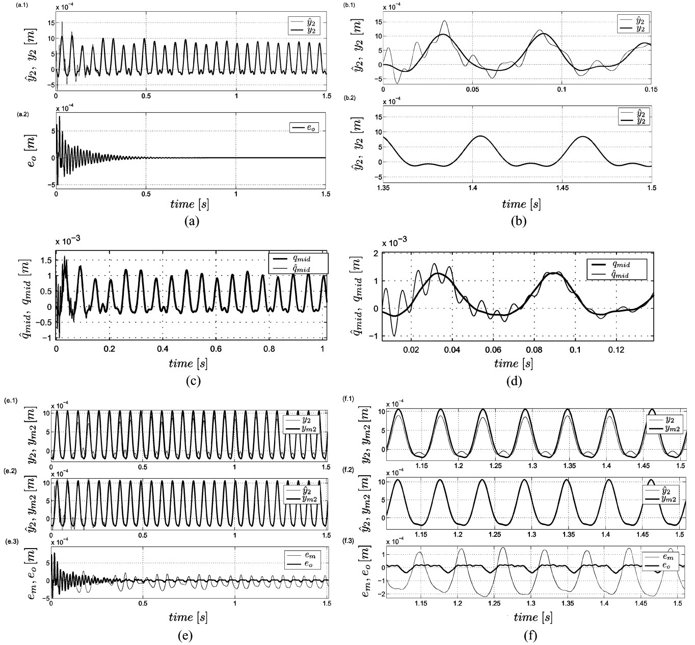
Fig. 3. (a.1) Model prediction y_2 [m] and observer reconstruction \hat{y}_2 [m]. (a.2) Estimation error e_o [m]. (b.1) Zoomed version of (a.1) in the transient state. (b.2) Zoomed version of (a.1) in steady-state. (c) Model prediction q_{mid} [m] and observer reconstruction \hat{q}_{mid} [m]. (d) Zoomed version of (c) in the transient state. (e.1) Measured displacement y_{m2} [m] and model prediction y_2 [m]. (e.2) Measured displacement y_{m2} [m] and observer reconstruction \hat{y}_2 [m]. (e.3) Estimation error e_o [m] and model error e_m [m]. (f.1) Zoomed version of (e.1). (f.2) Zoomed version of (e.2). (f.3) Zoomed version of (e.3). The excitation frequency is \omega/2\pi = 35 Hz and the excitation amplitude is u_0 = 50 N.
